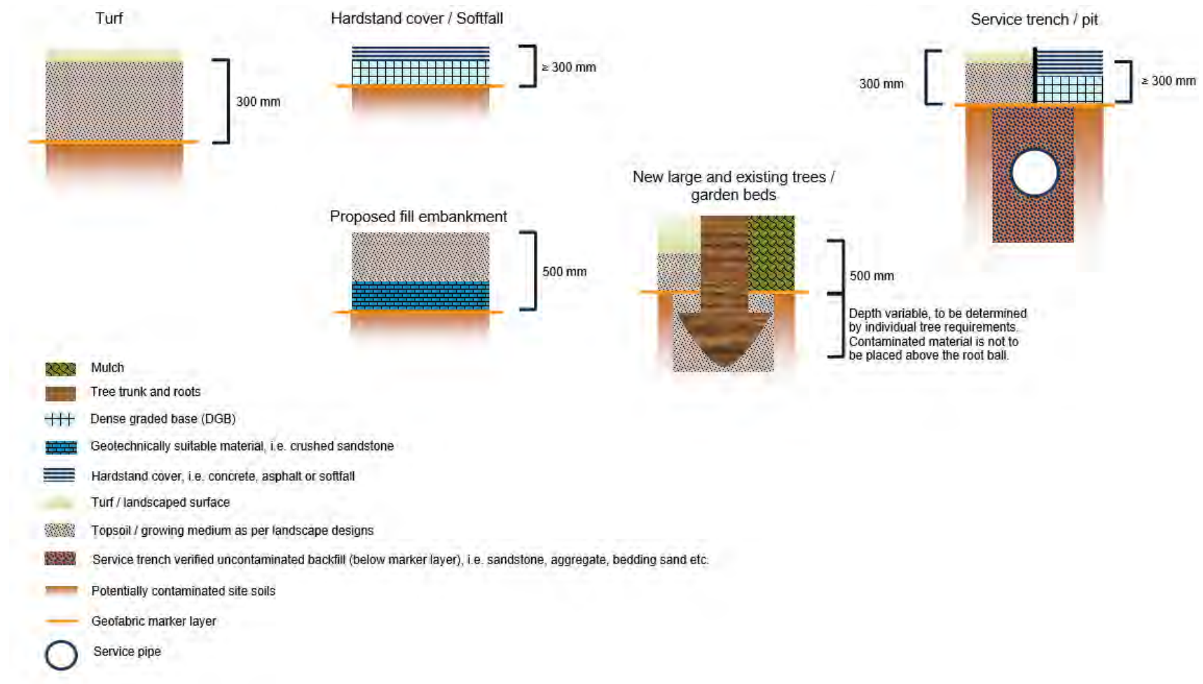
Figure 12-1 Containment / Encapsulation, Conceptual Cross-Sections
